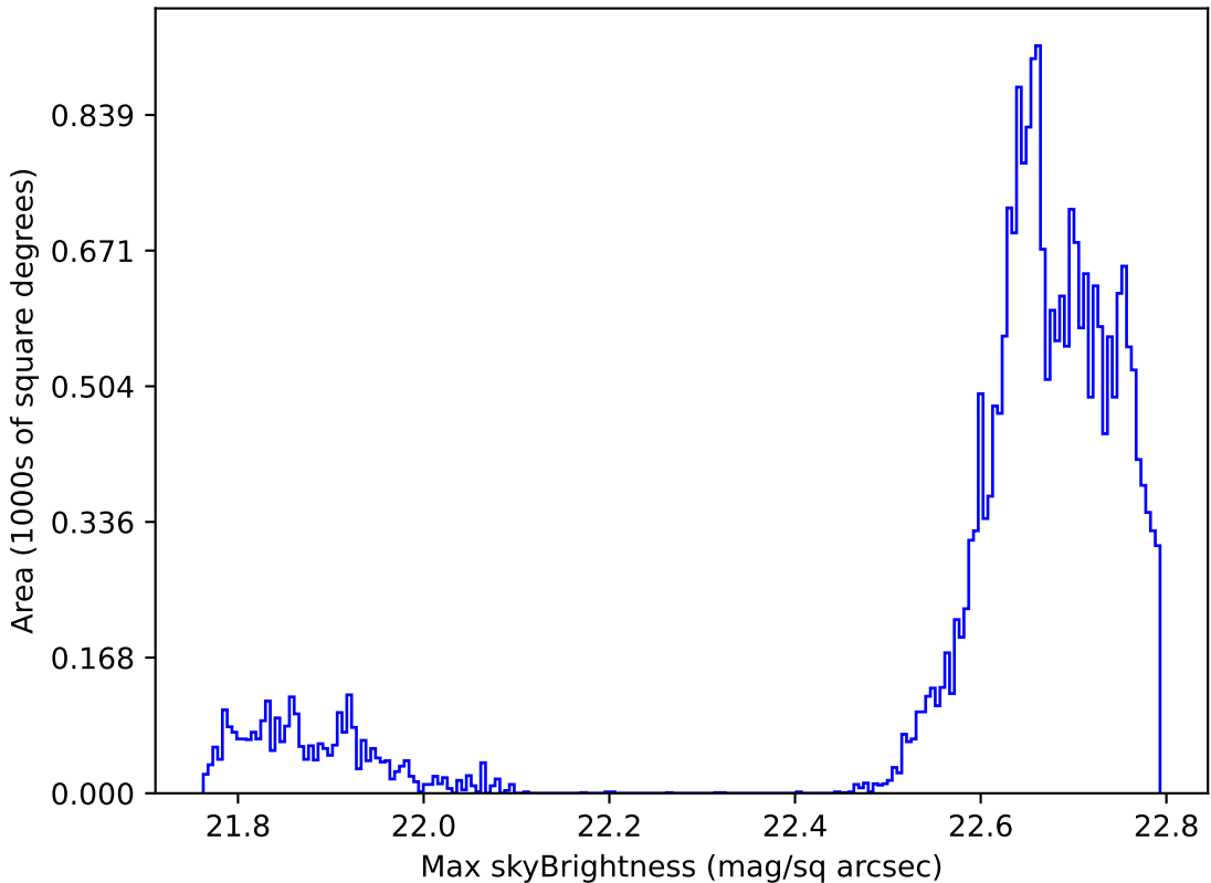
mw_roll_bulge_v3.3_10yrs Yr 1 all bands: Max skyBrightness
