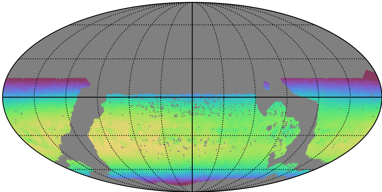
mw_roll_bulge_v3.3_10yrs WFD z band: Max skyBrightness
