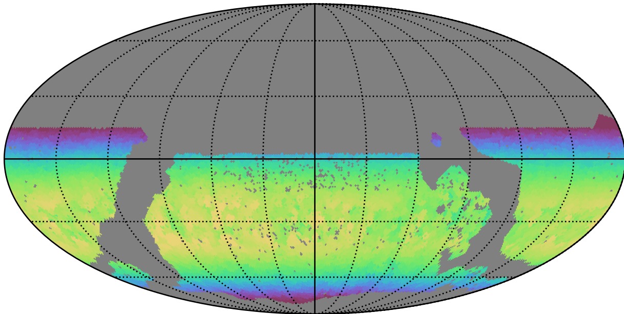
mw_roll_bulge_v3.3_10yrs WFD y band: Max skyBrightness
