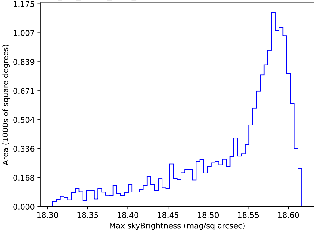
mw_roll_bulge_v3.3_10yrs WFD y band: Max skyBrightness
