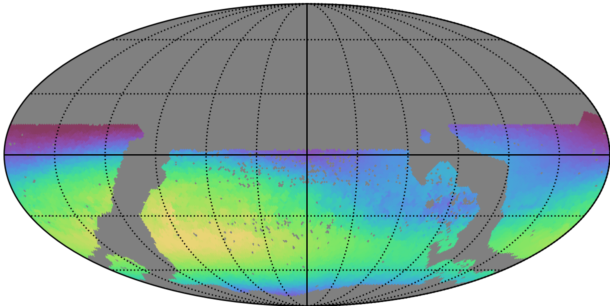
mw_roll_bulge_v3.3_10yrs WFD u band: Max skyBrightness
