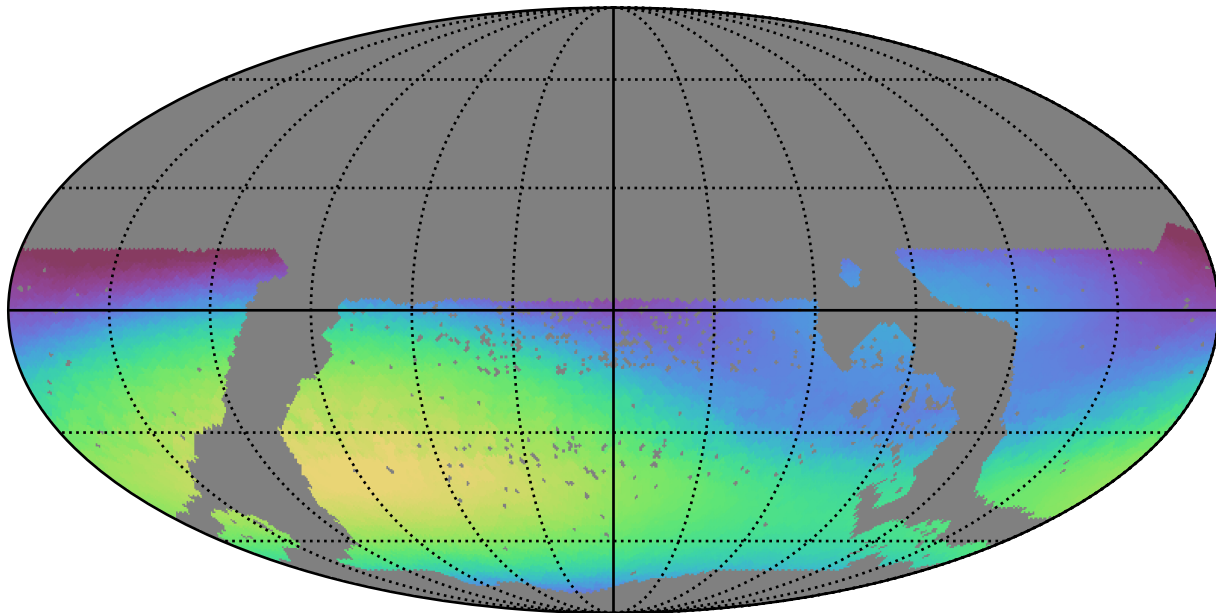
mw_roll_bulge_v3.3_10yrs WFD r band: Max skyBrightness
