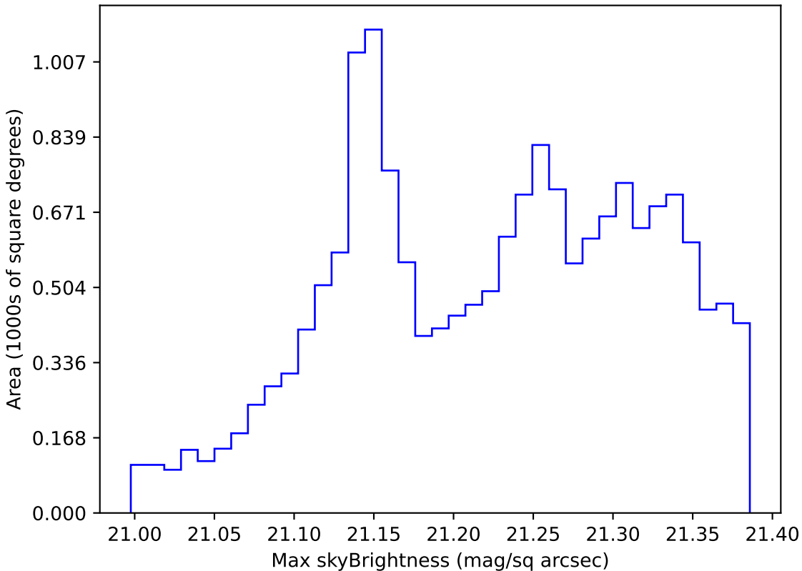
mw_roll_bulge_v3.3_10yrs WFD r band: Max skyBrightness
