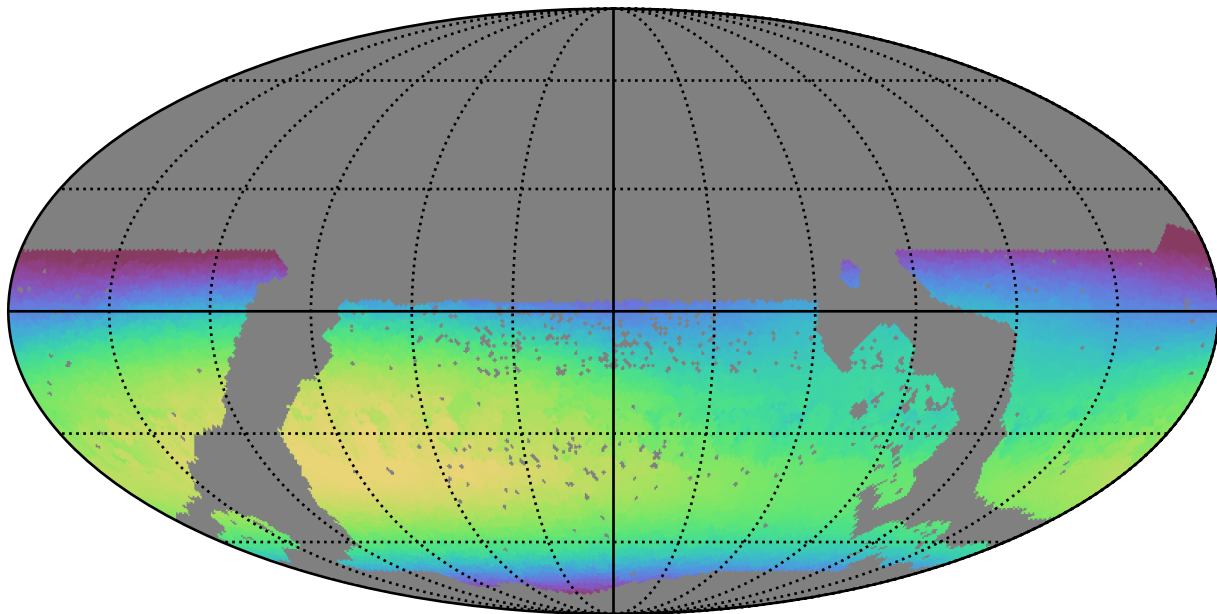
mw_roll_bulge_v3.3_10yrs WFD i band: Max skyBrightness
