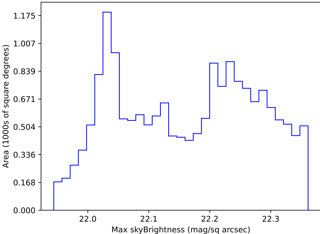
mw_roll_bulge_v3.3_10yrs WFD g band: Max skyBrightness
