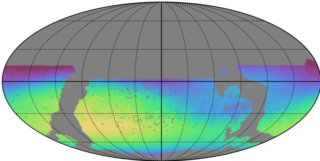
mw_roll_bulge_v3.3_10yrs WFD all bands: Max skyBrightness
