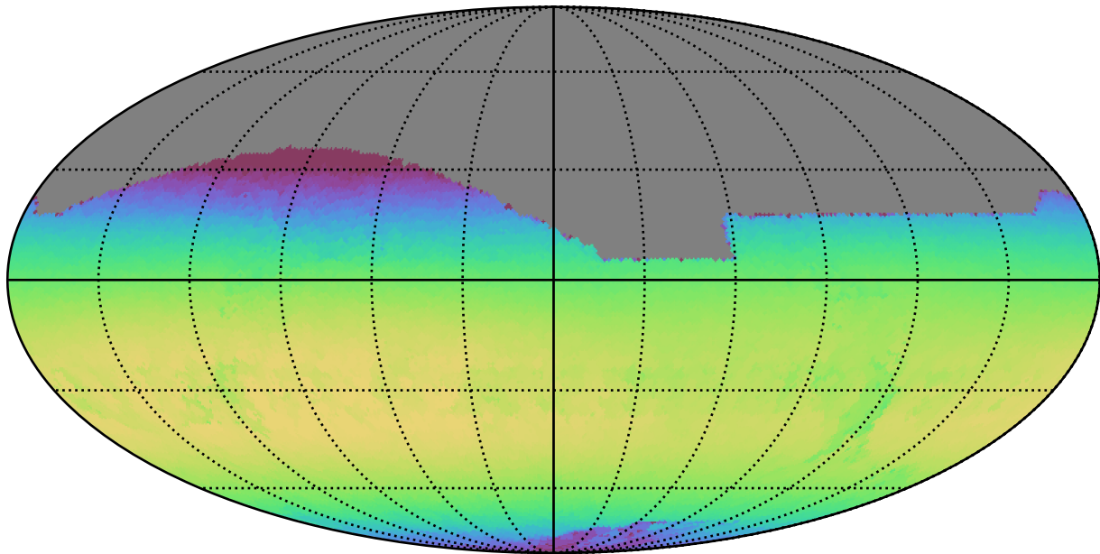
mw_roll_bulge_v3.3_10yrs All sky z band: Max skyBrightness
