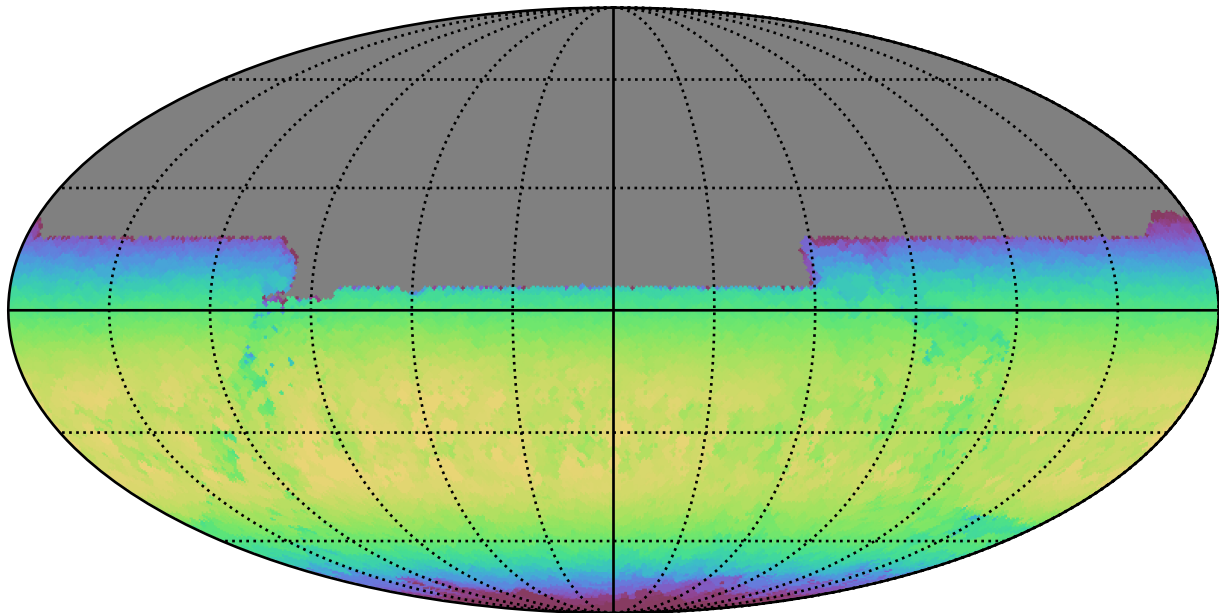
mw_roll_bulge_v3.3_10yrs All sky y band: Max skyBrightness
