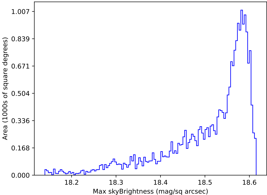
mw_roll_bulge_v3.3_10yrs All sky y band: Max skyBrightness
