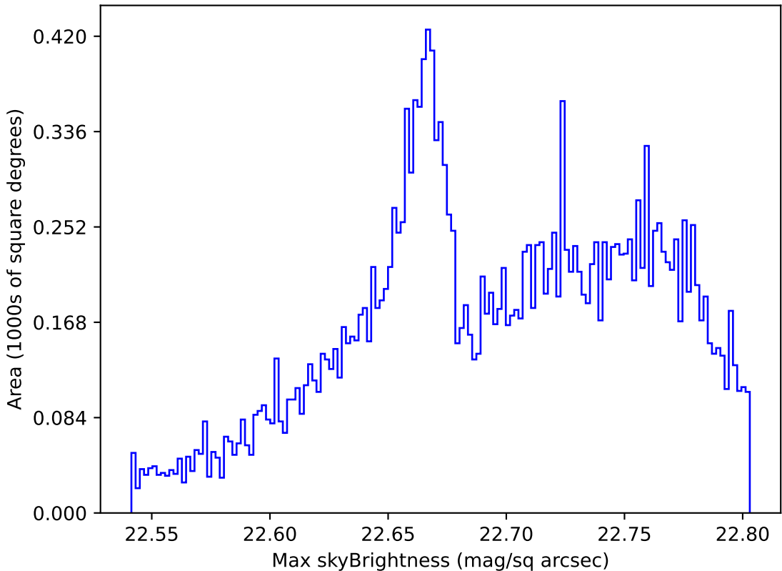
mw_roll_bulge_v3.3_10yrs All sky u band: Max skyBrightness
