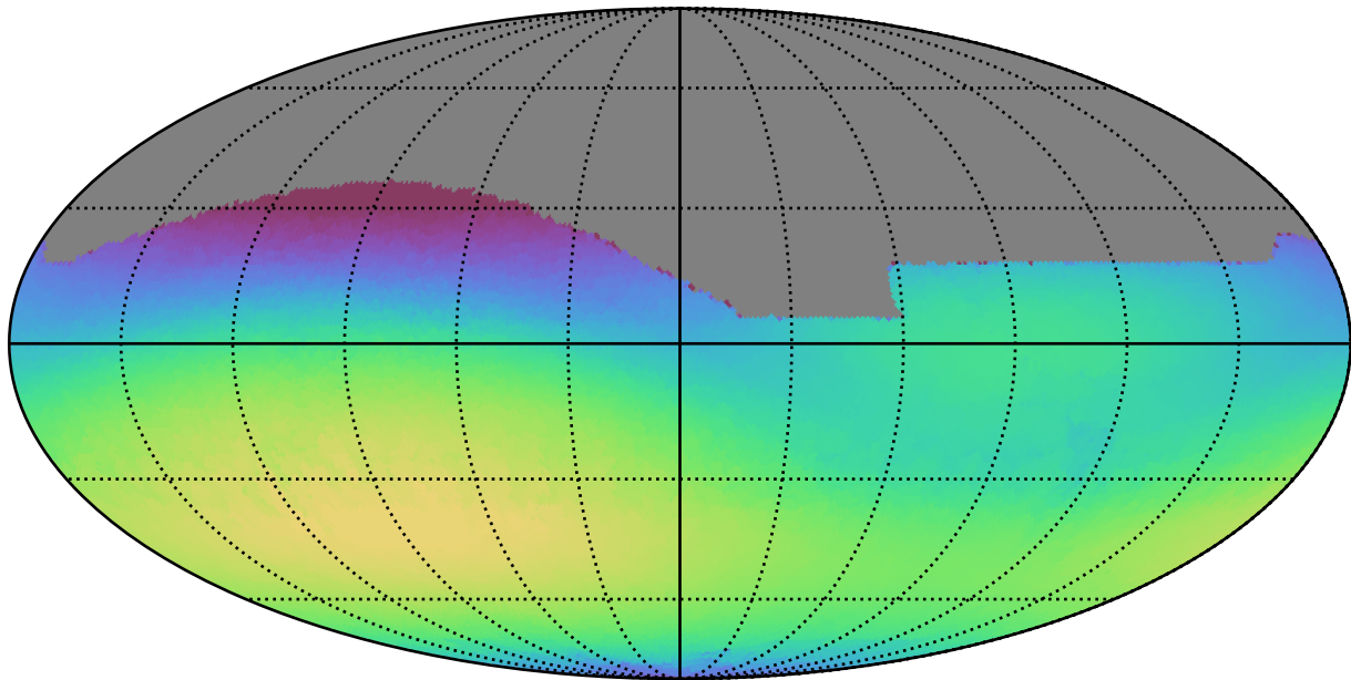
mw_roll_bulge_v3.3_10yrs All sky r band: Max skyBrightness
