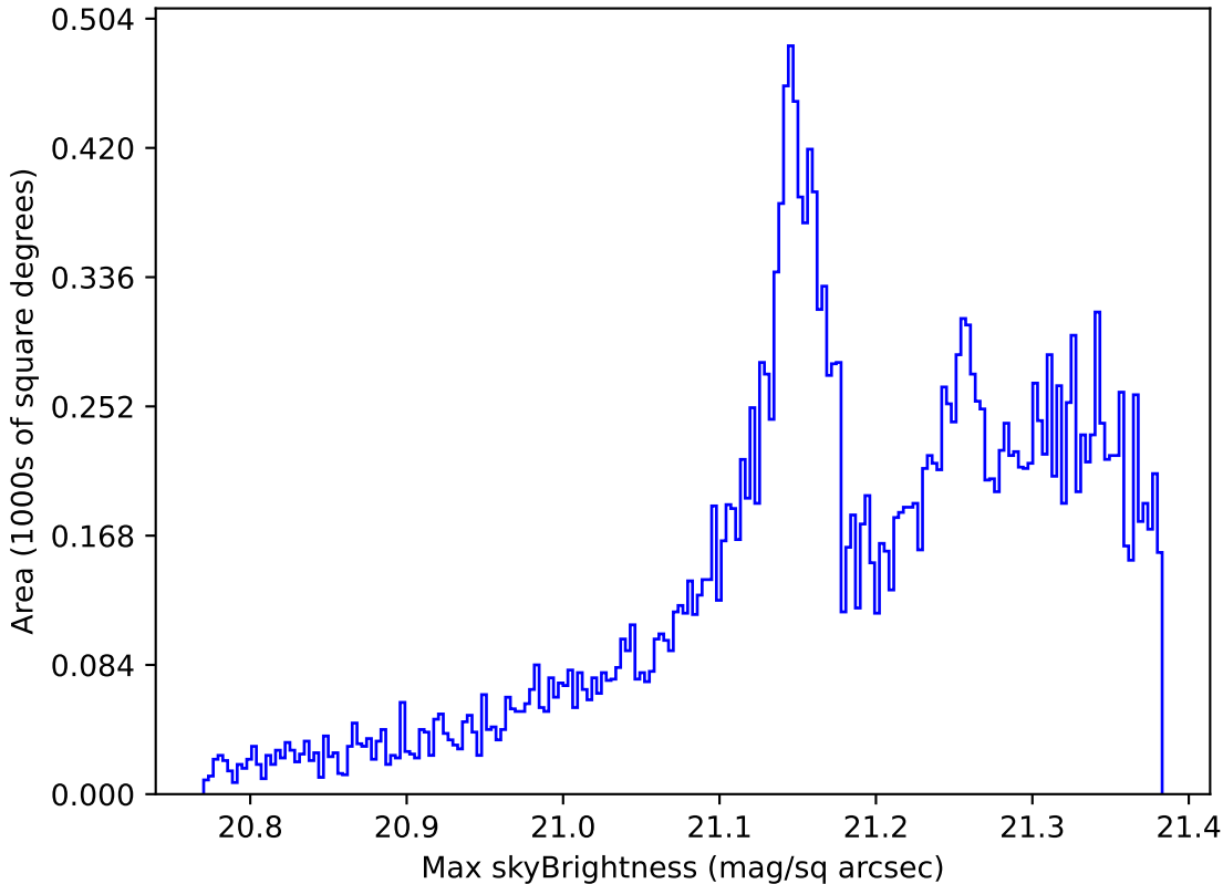
mw_roll_bulge_v3.3_10yrs All sky r band: Max skyBrightness
