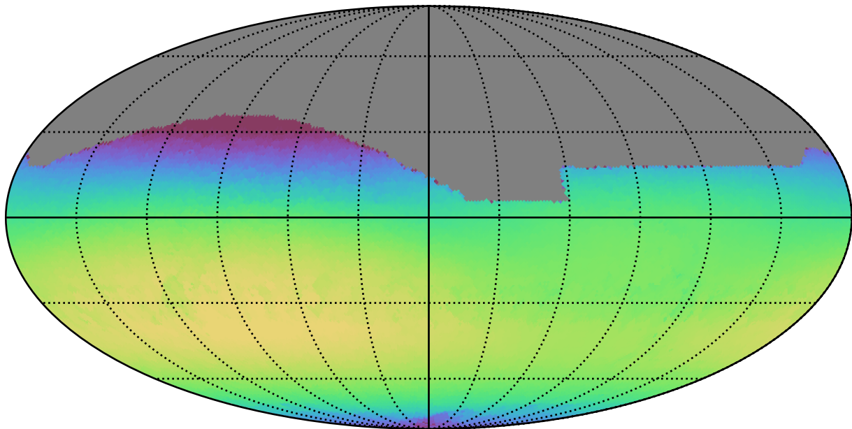
mw_roll_bulge_v3.3_10yrs All sky i band: Max skyBrightness
