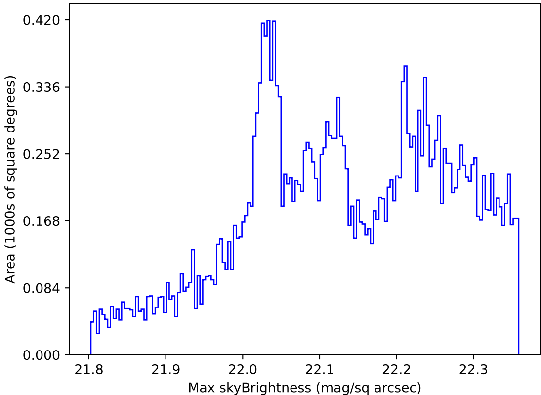
mw_roll_bulge_v3.3_10yrs All sky g band: Max skyBrightness
