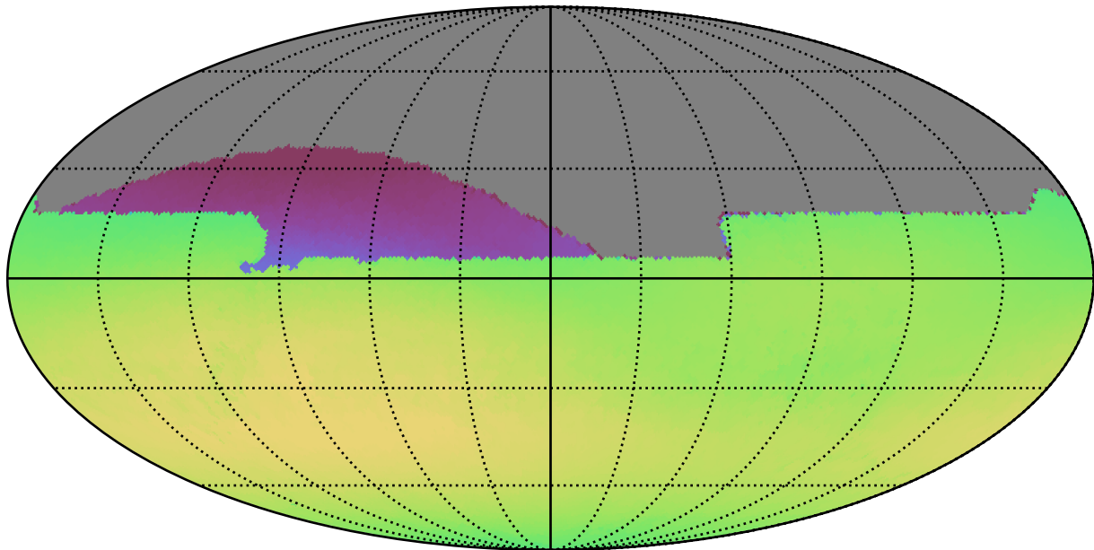
mw_roll_bulge_v3.3_10yrs All sky all bands: Max skyBrightness
