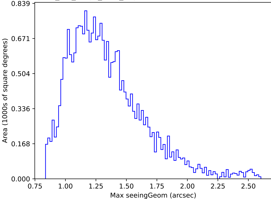
mw_roll_bulge_v3.3_10yrs Yr 1 i band: Max seeingGeom
