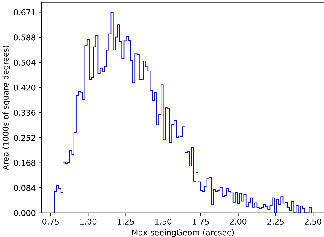
mw_roll_bulge_v3.3_10yrs Yr 1 g band: Max seeingGeom
