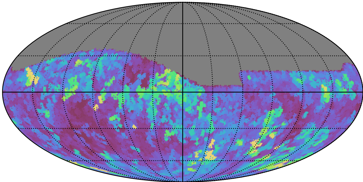
mw_roll_bulge_v3.3_10yrs Yr 1 all bands: Max seeingGeom
