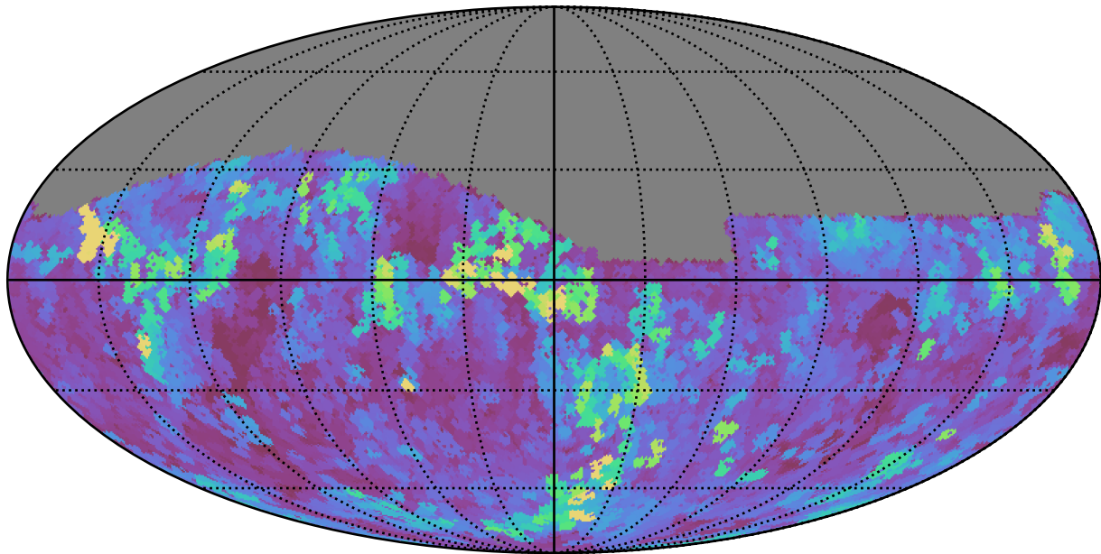
mw_roll_bulge_v3.3_10yrs Yr 1 z band: Max seeingEff
