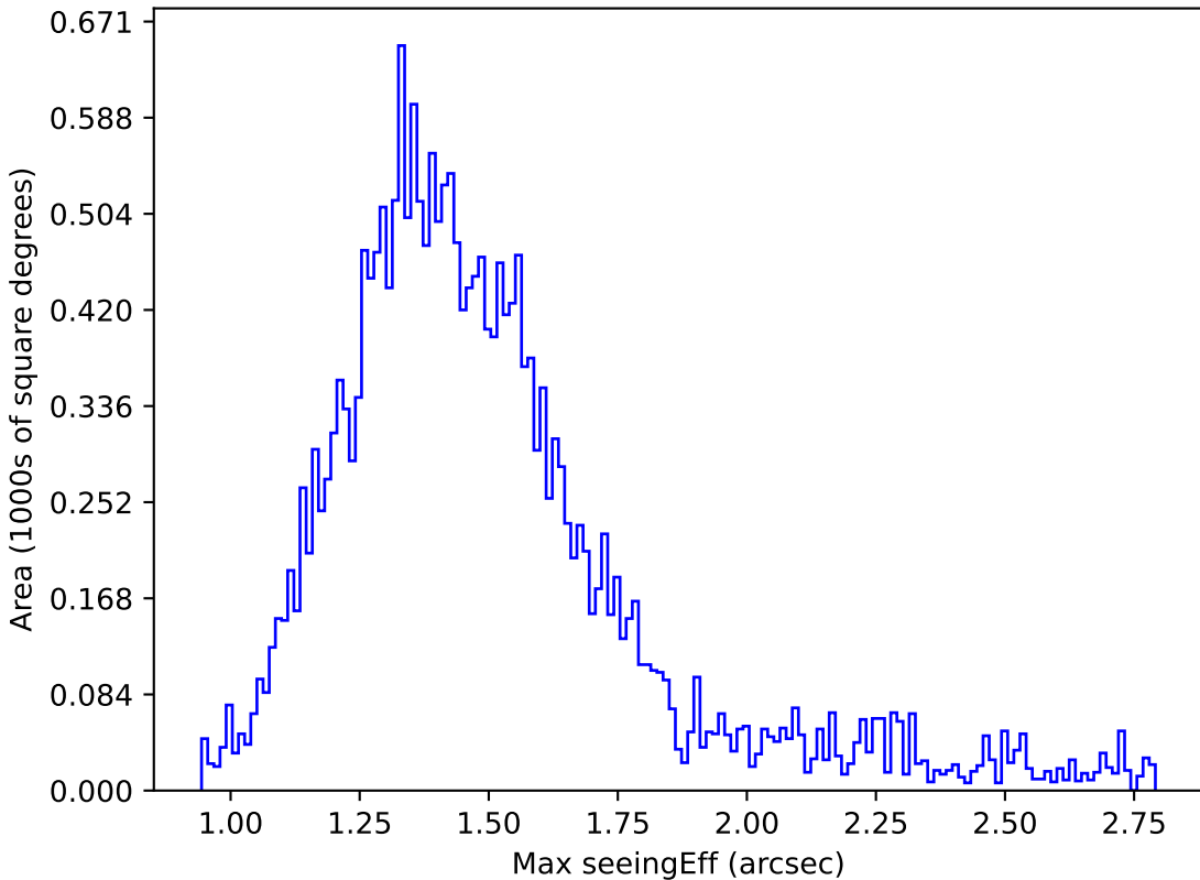
mw_roll_bulge_v3.3_10yrs Yr 1 y band: Max seeingEff
