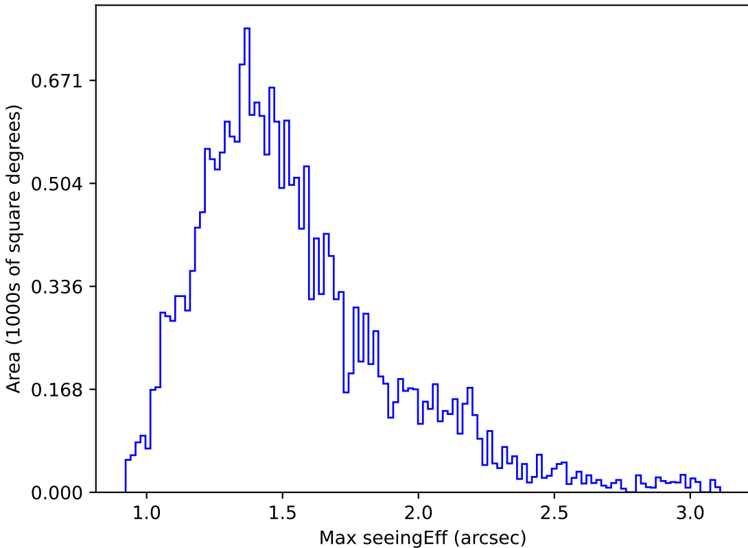
mw_roll_bulge_v3.3_10yrs Yr 1 u band: Max seeingEff
