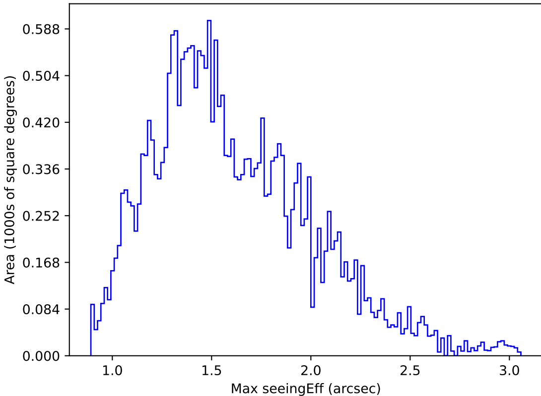
mw_roll_bulge_v3.3_10yrs Yr 1 r band: Max seeingEff
