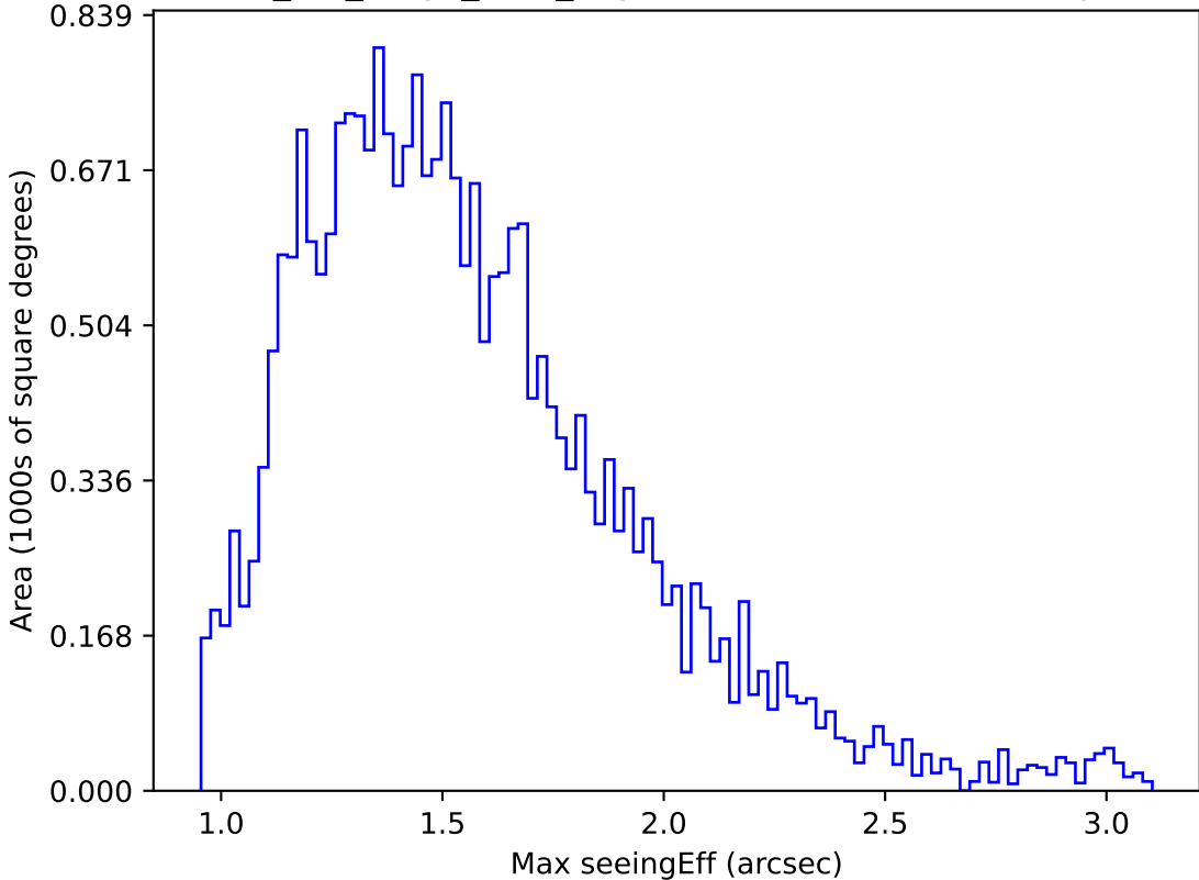
mw_roll_bulge_v3.3_10yrs Yr 1 i band: Max seeingEff
