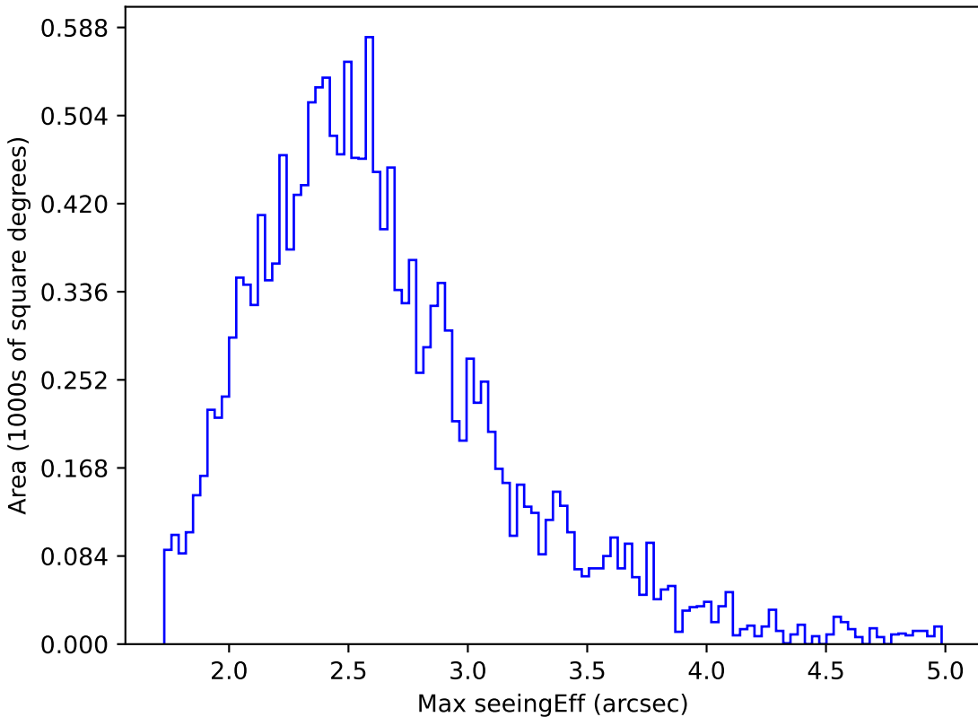
mw_roll_bulge_v3.3_10yrs WFD z band: Max seeingEff
