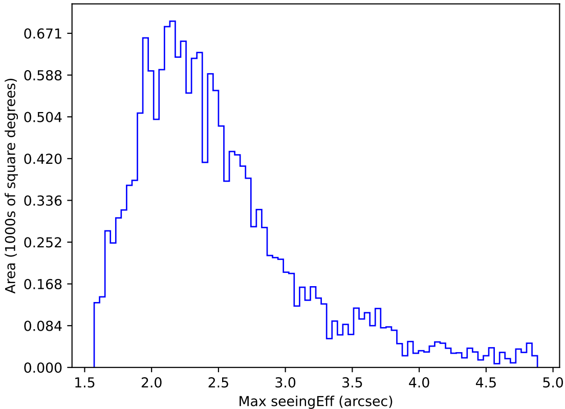
mw_roll_bulge_v3.3_10yrs WFD y band: Max seeingEff
