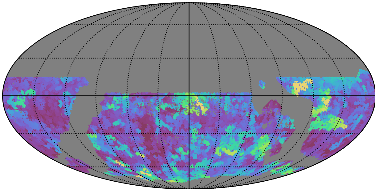
mw_roll_bulge_v3.3_10yrs WFD u band: Max seeingEff
