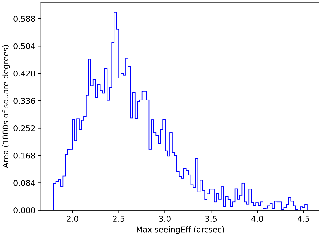
mw_roll_bulge_v3.3_10yrs WFD r band: Max seeingEff
