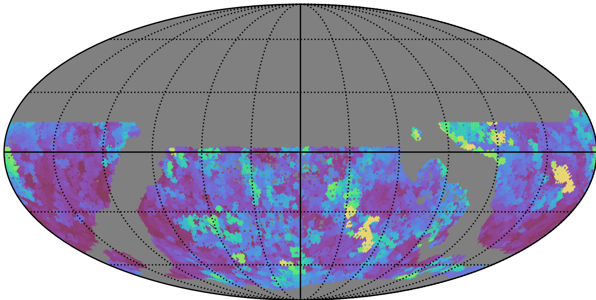
mw_roll_bulge_v3.3_10yrs WFD i band: Max seeingEff
