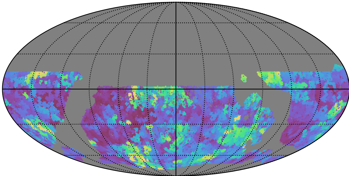
mw_roll_bulge_v3.3_10yrs WFD g band: Max seeingEff
