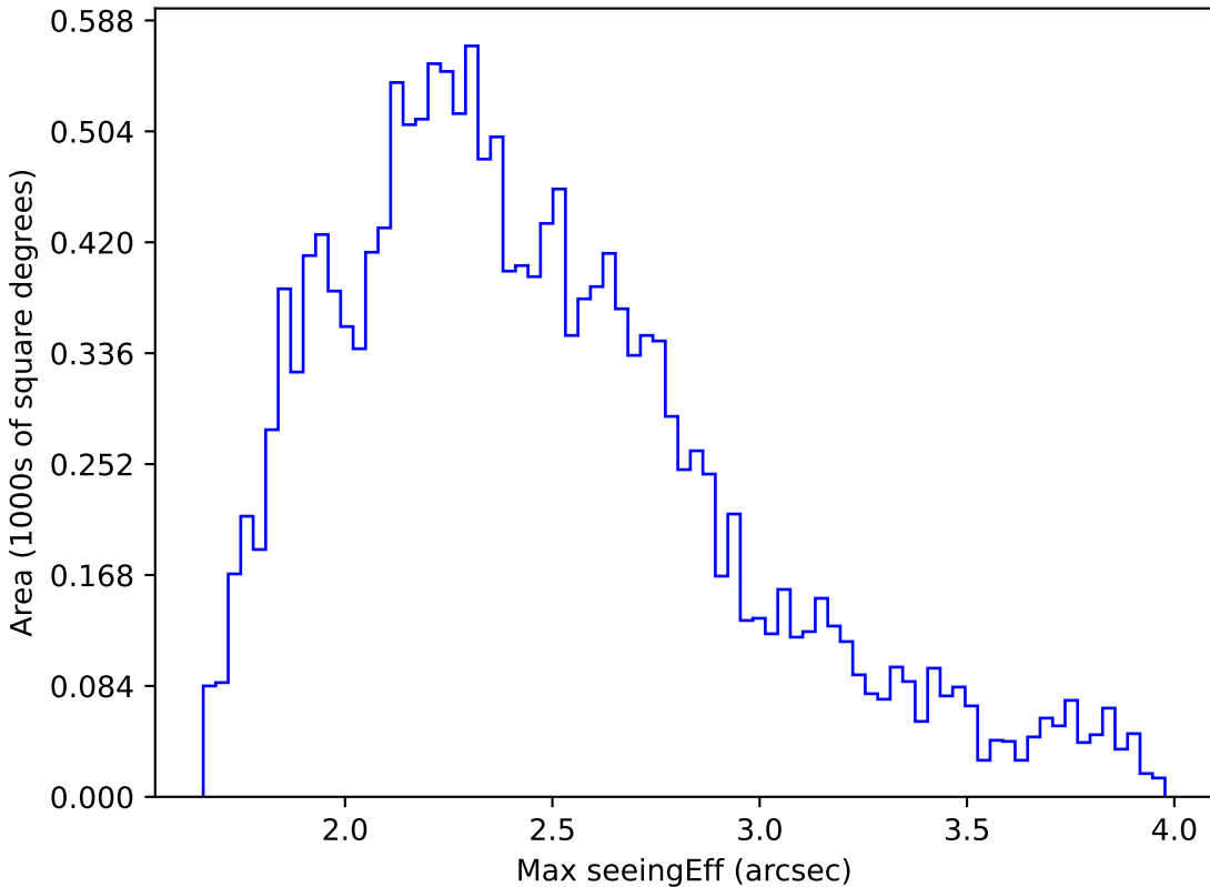
mw_roll_bulge_v3.3_10yrs WFD g band: Max seeingEff
