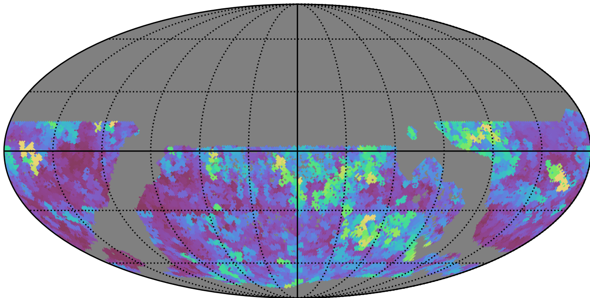
mw_roll_bulge_v3.3_10yrs WFD all bands: Max seeingEff
