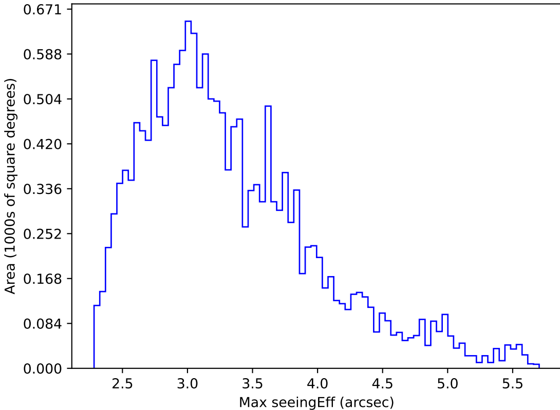
mw_roll_bulge_v3.3_10yrs WFD all bands: Max seeingEff
