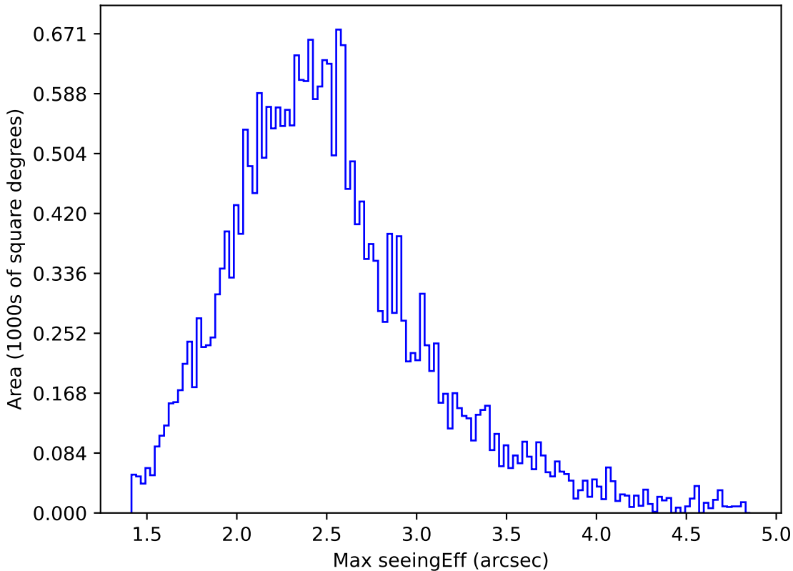
mw_roll_bulge_v3.3_10yrs All sky z band: Max seeingEff
