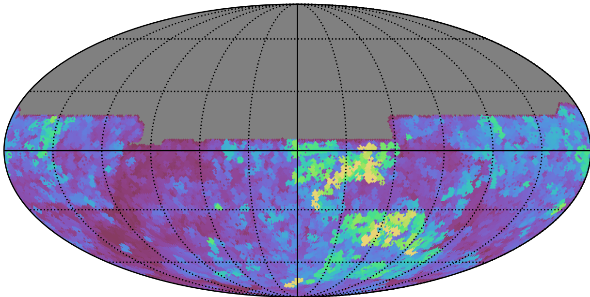
mw_roll_bulge_v3.3_10yrs All sky y band: Max seeingEff
