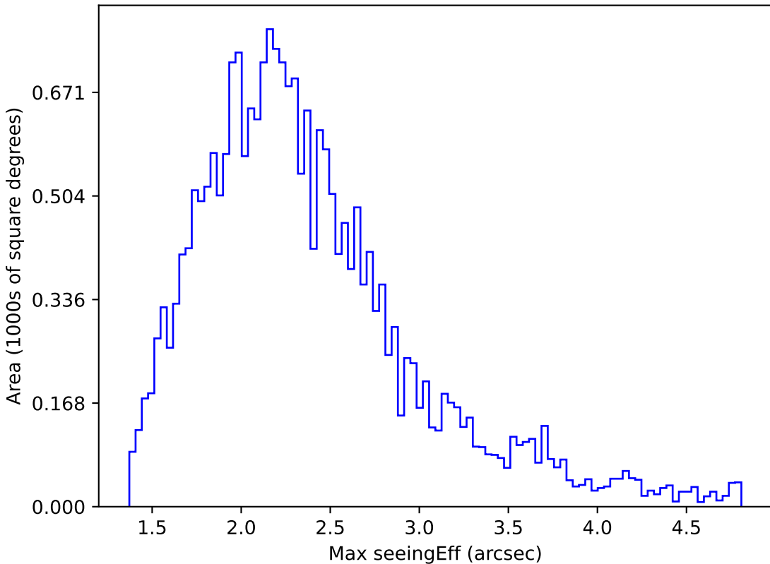
mw_roll_bulge_v3.3_10yrs All sky y band: Max seeingEff
