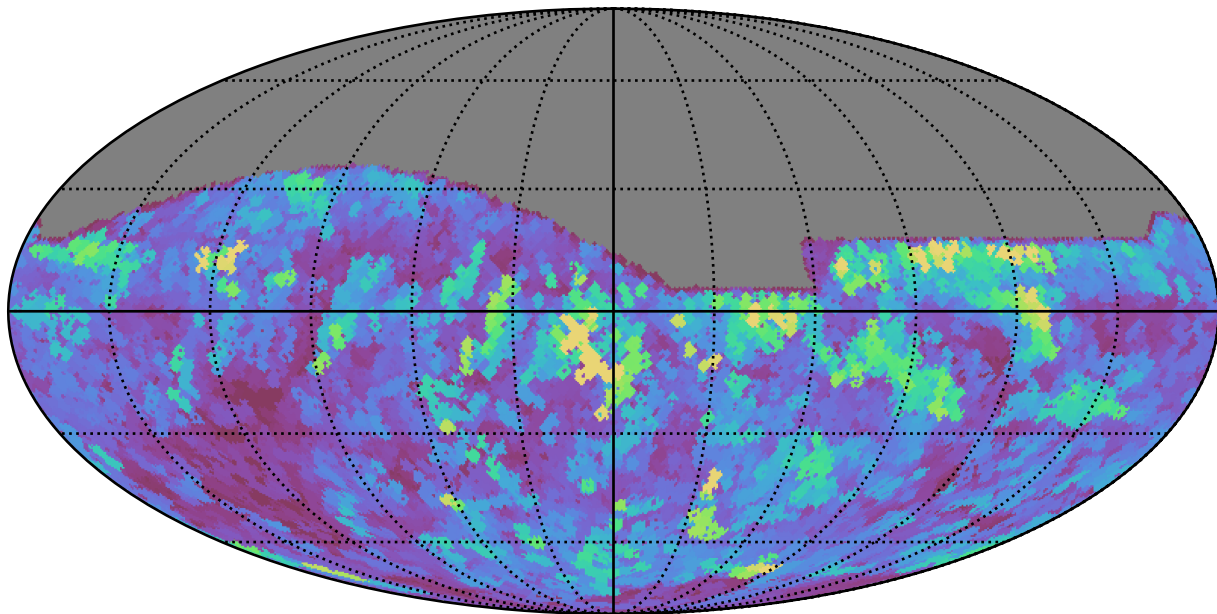
mw_roll_bulge_v3.3_10yrs All sky r band: Max seeingEff
