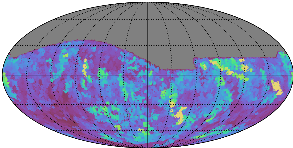
mw_roll_bulge_v3.3_10yrs All sky i band: Max seeingEff
