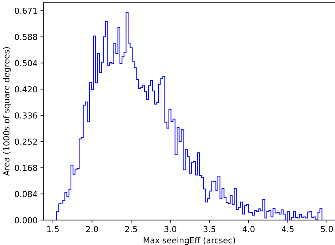
mw_roll_bulge_v3.3_10yrs All sky i band: Max seeingEff
