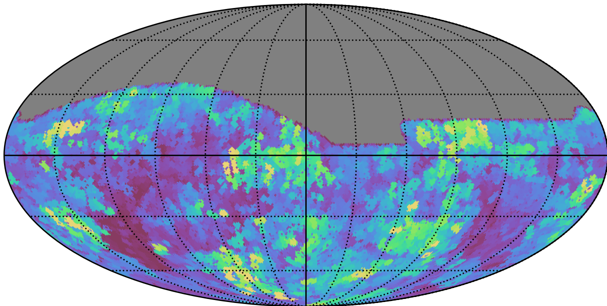
mw_roll_bulge_v3.3_10yrs All sky g band: Max seeingEff
