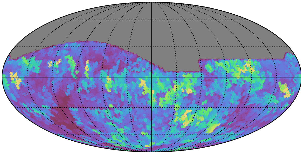
mw_roll_bulge_v3.3_10yrs All sky all bands: Max seeingEff
