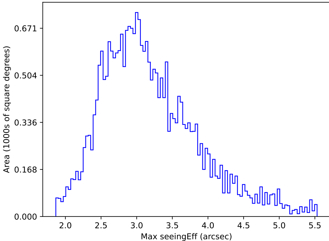
mw_roll_bulge_v3.3_10yrs All sky all bands: Max seeingEff
