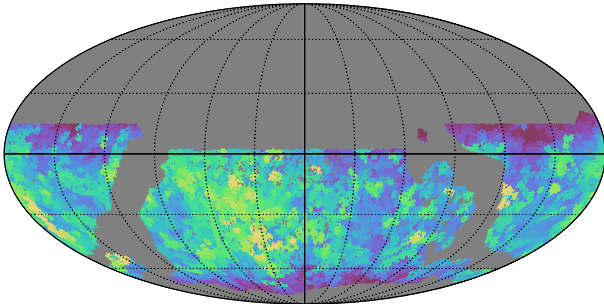
mw_roll_bulge_v3.3_10yrs WFD all bands: Max saturation_mag
