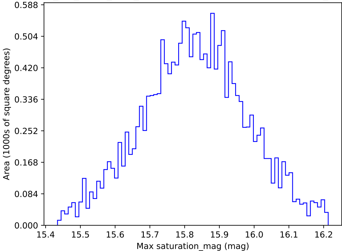
mw_roll_bulge_v3.3_10yrs WFD all bands: Max saturation_mag
