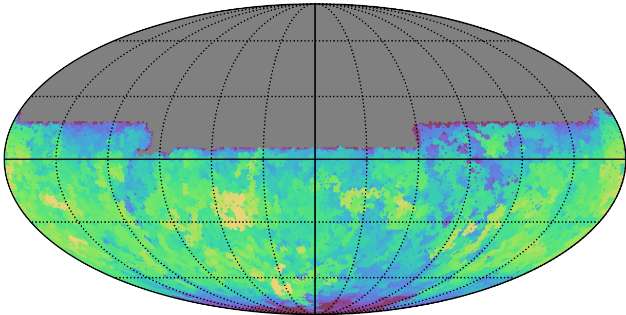
mw_roll_bulge_v3.3_10yrs All sky u band: Max saturation_mag
