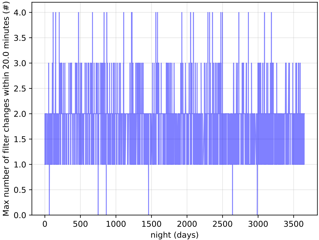
mw_roll_bulge_v3.3_10yrs Per Night: Max number of filter changes within 20.0 minutes
