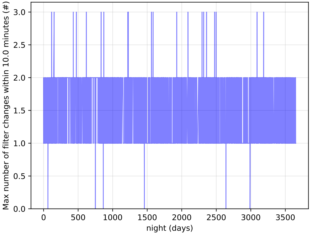
mw_roll_bulge_v3.3_10yrs Per Night: Max number of filter changes within 10.0 minutes
